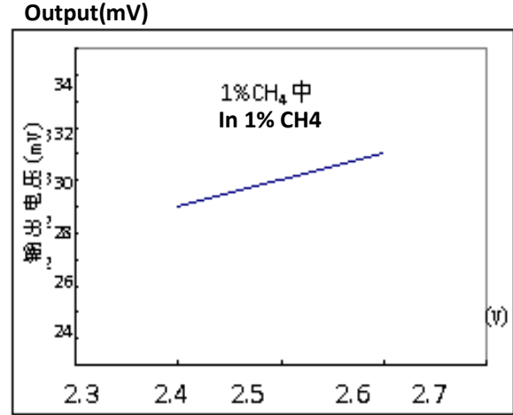
Fig9. Sensitivity with different voltage
