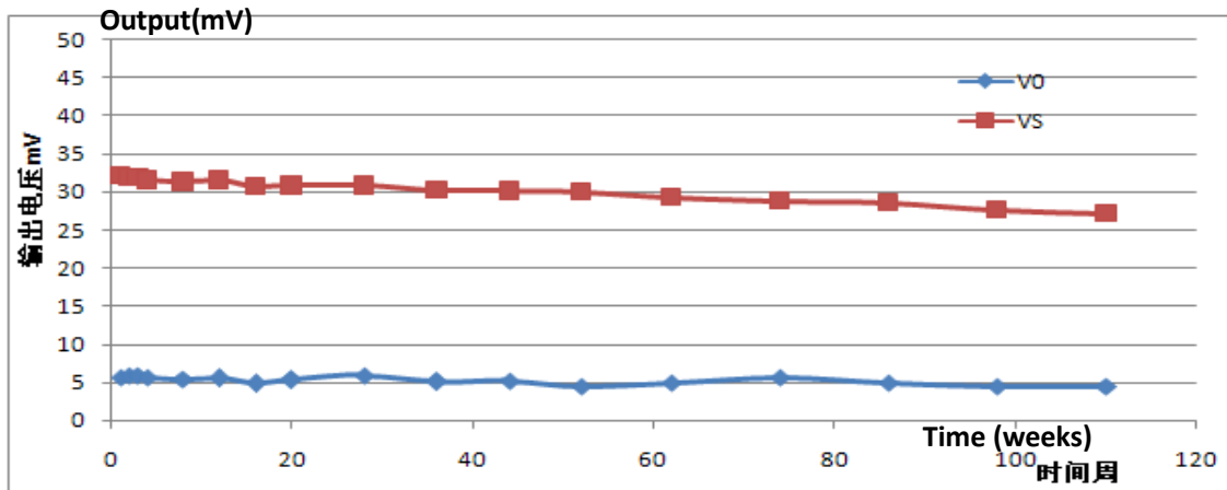
Fig10. Sensitivity fluctuation
